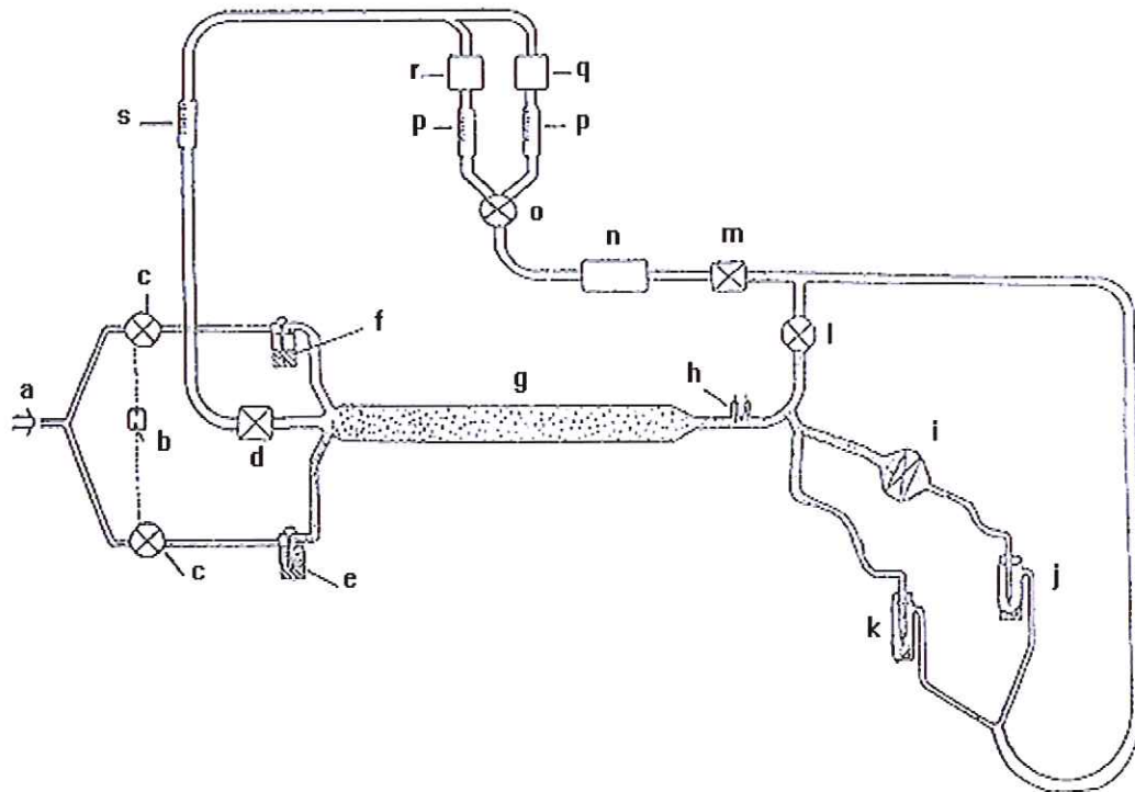
FIGURE 1. HENDERSON APPARATUS FOR CHALLENGING FILTERS WITH MICROBIAL AEROSOLS
